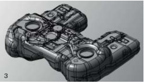
3. Optional: self-sealing tank coated inside with an anti-explosive material.
